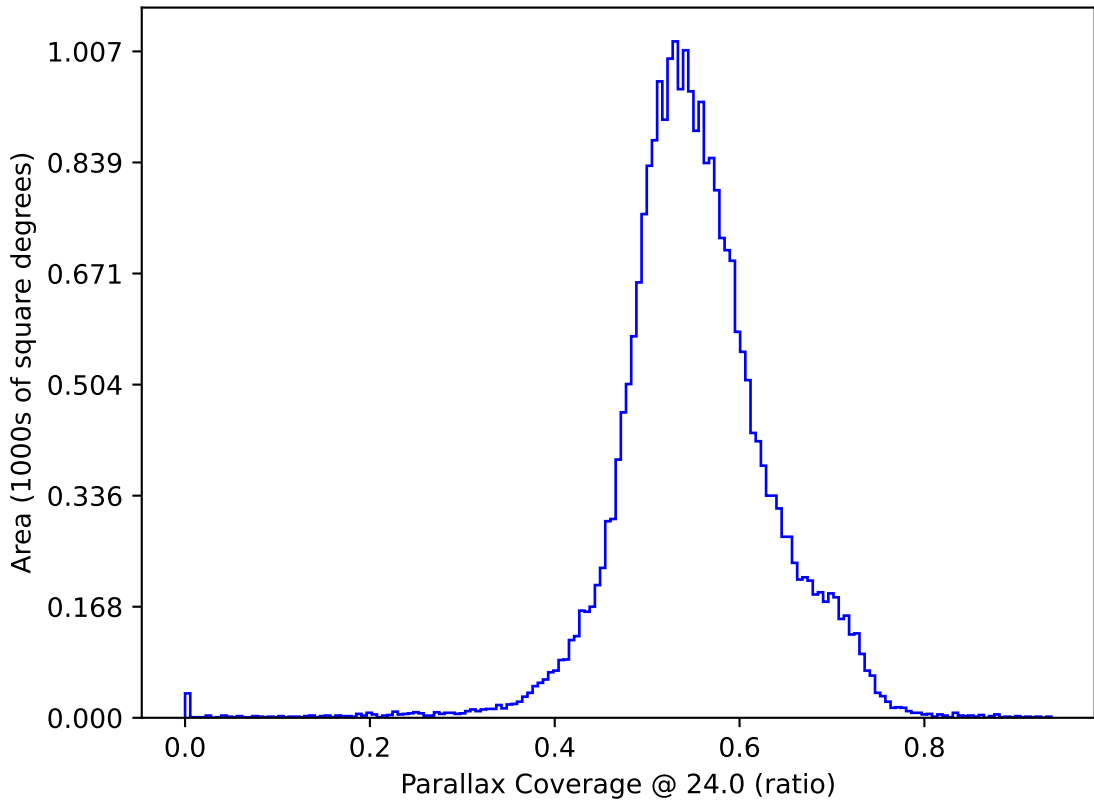
too_elab_heavy_r128_d3_gz_v3.4_10yrs : Parallax Coverage @ 24.0
