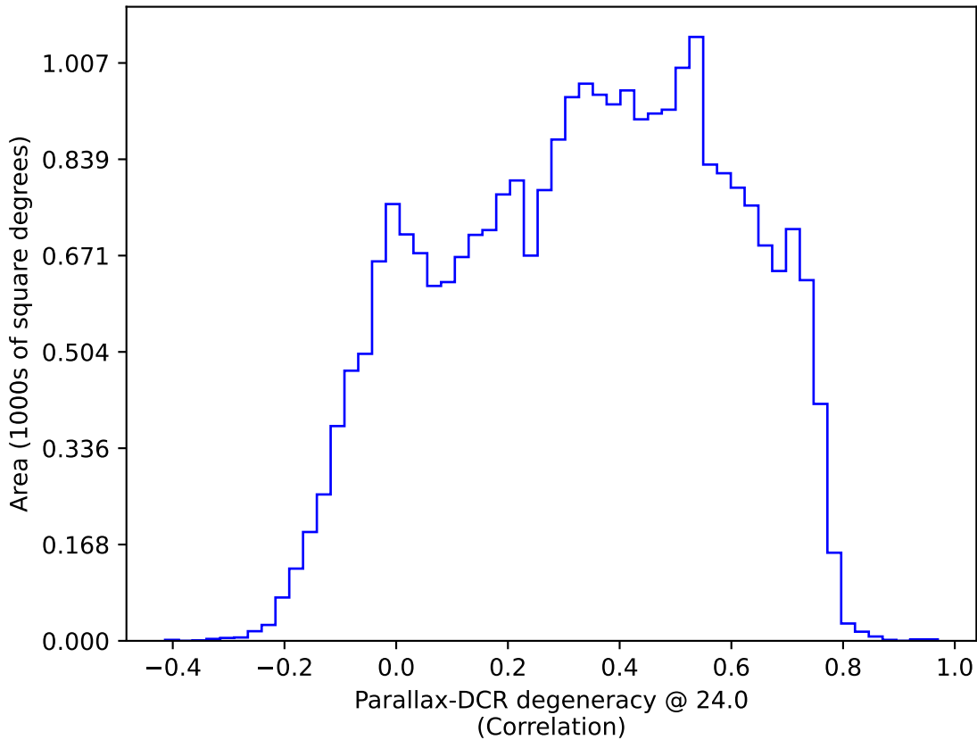
too_elab_heavy_r128_d3_gz_v3.4_10yrs : Parallax-DCR degeneracy @ 24.0
