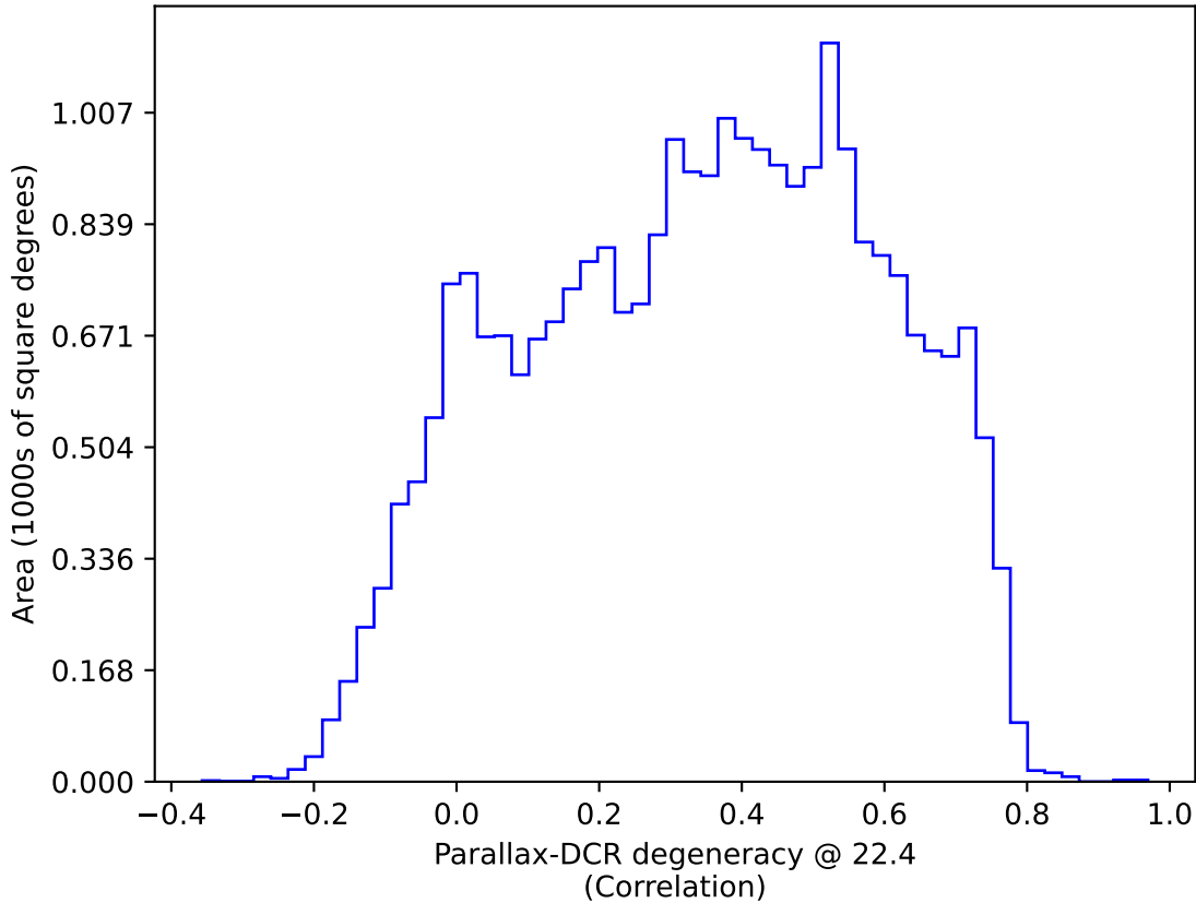
too_elab_heavy_r128_d3_gz_v3.4_10yrs : Parallax-DCR degeneracy @ 22.4
