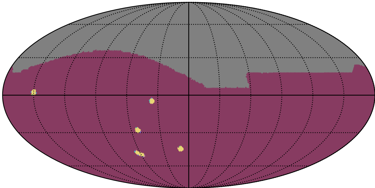
too_elab_heavy_r128_d3_gz_v3.4_10yrs : NumberOfQuickRevisits
