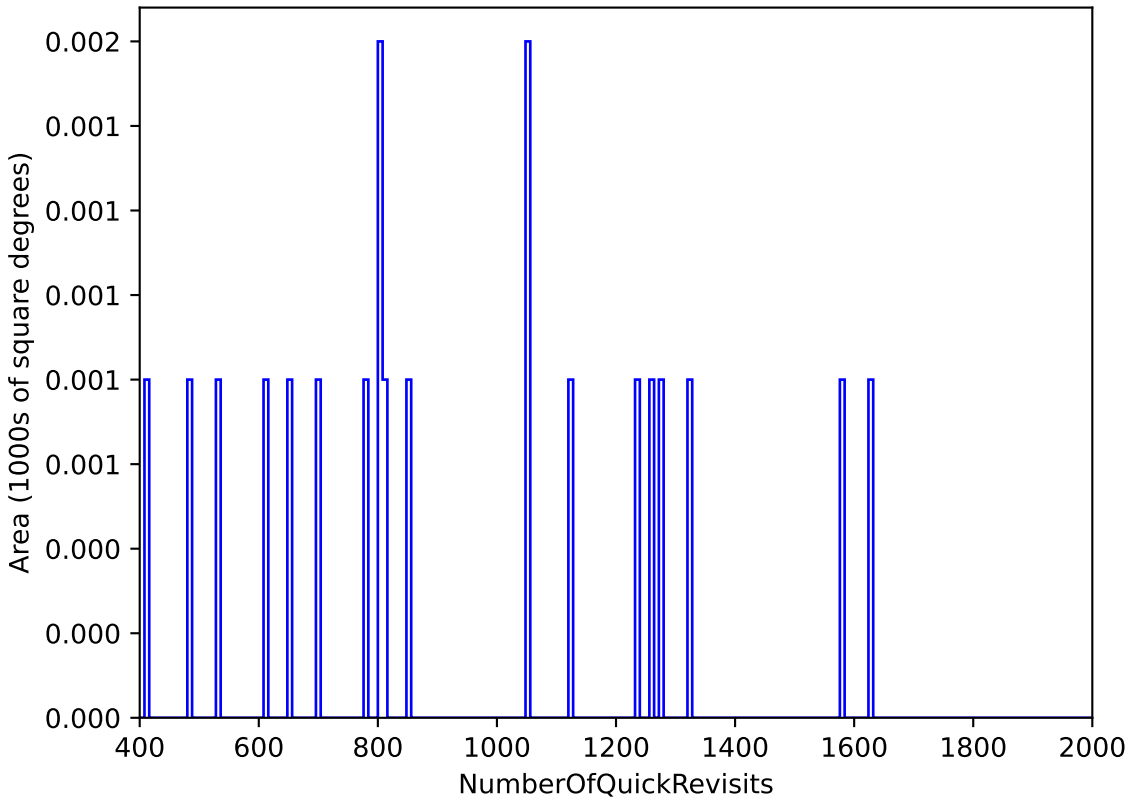
too_elab_heavy_r128_d3_gz_v3.4_10yrs : NumberOfQuickRevisits
