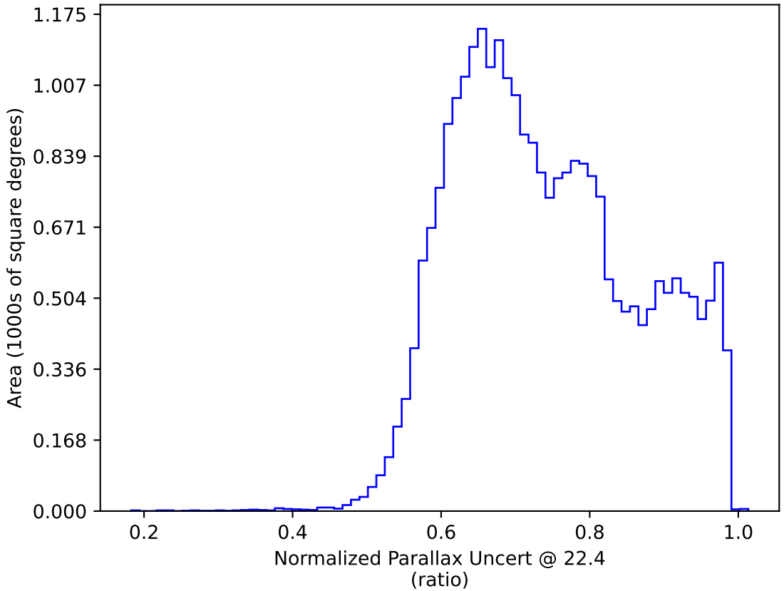
too_elab_heavy_r128_d3_gz_v3.4_10yrs : Normalized Parallax Uncert @ 22.4
