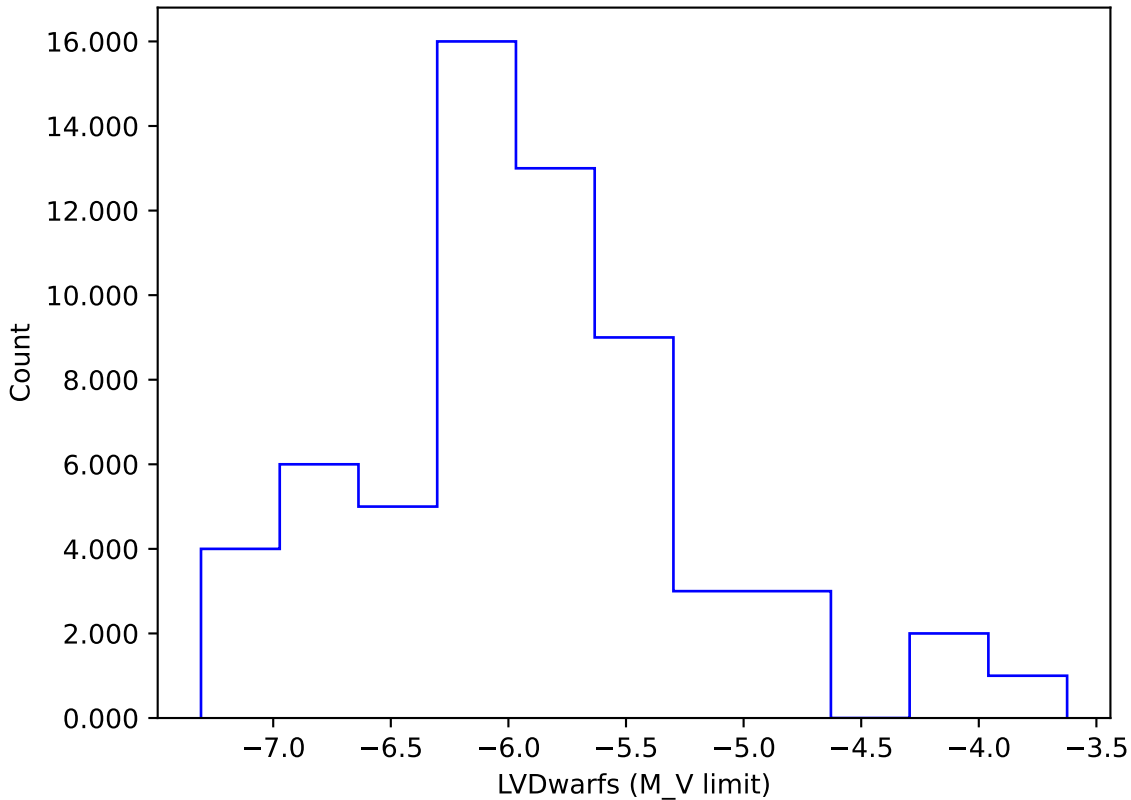
too_elab_heavy_r128_d3_gz_v3.4_10yrs gi: LVDwarfs
