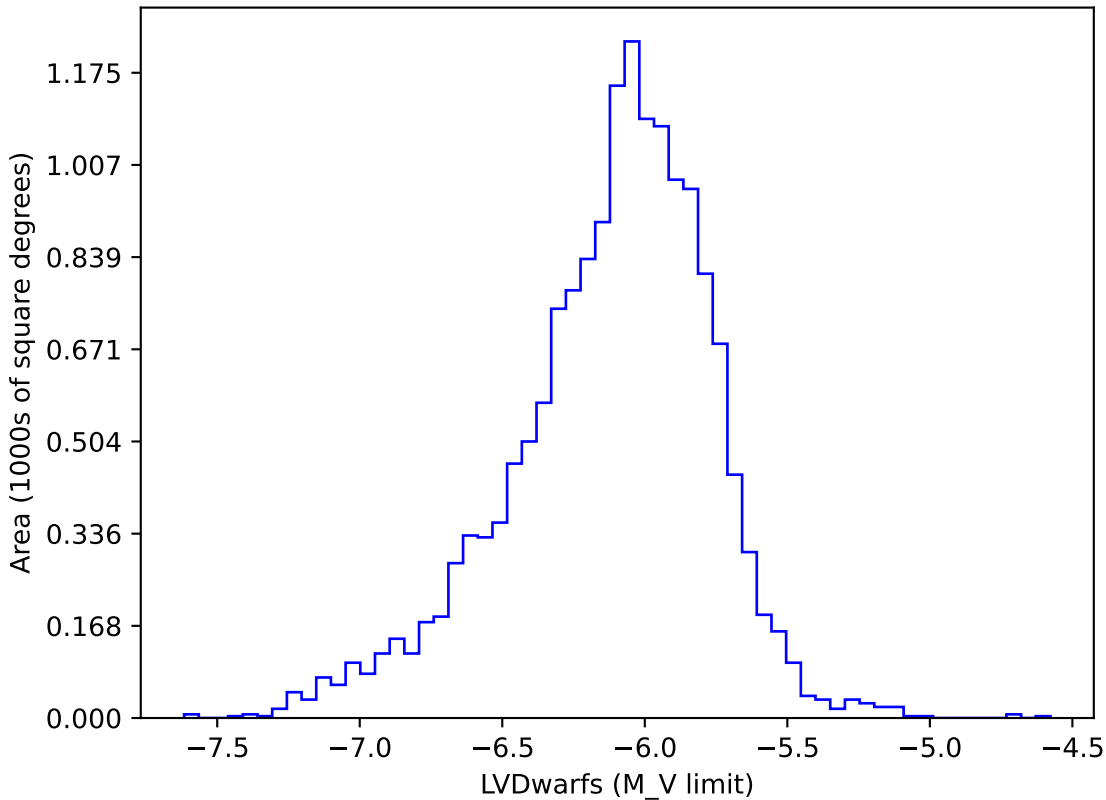
too_elab_heavy_r128_d3_gz_v3.4_10yrs gi: LVDwarfs
