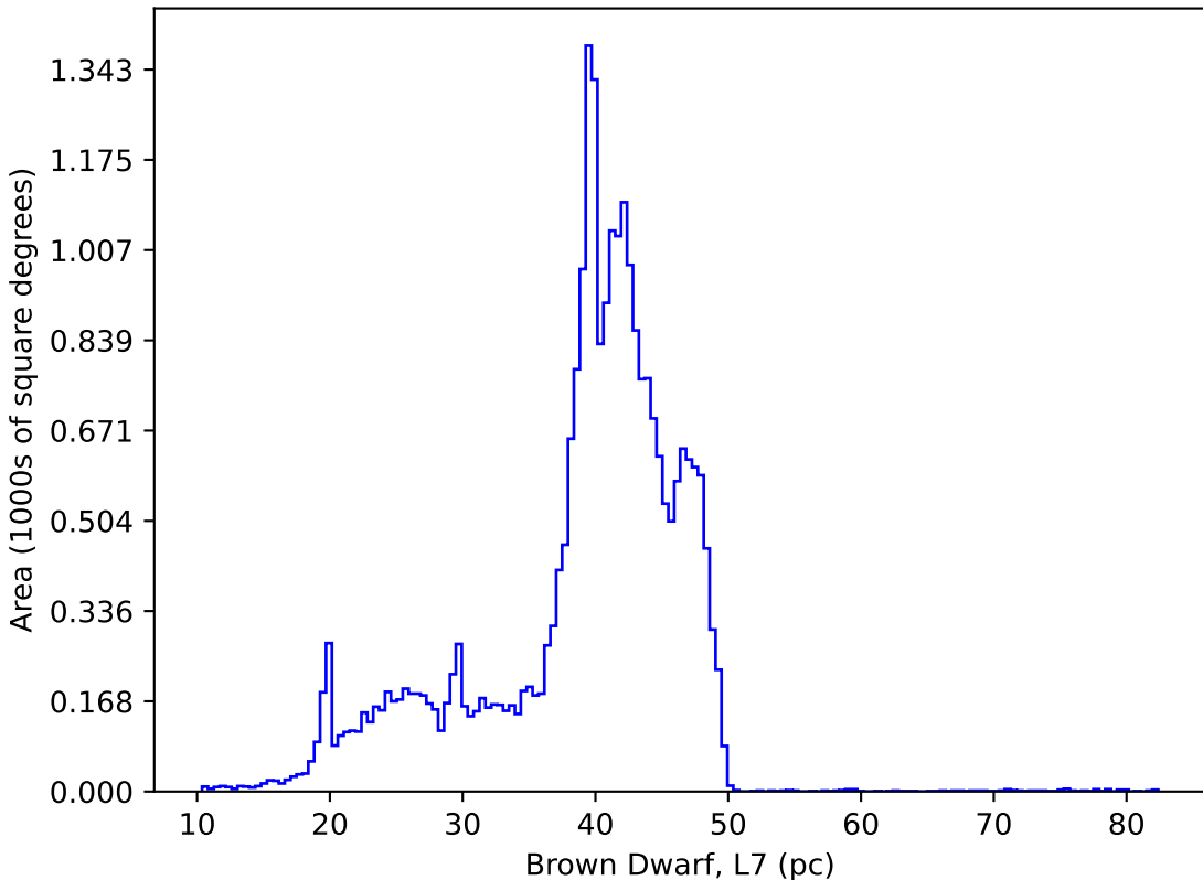
too_elab_heavy_r128_d3_gz_v3.4_10yrs : Brown Dwarf, L7
