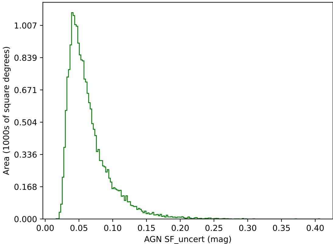
too_elab_heavy_r128_d3_gz_v3.4_10yrs g band: AGN SF_uncert
