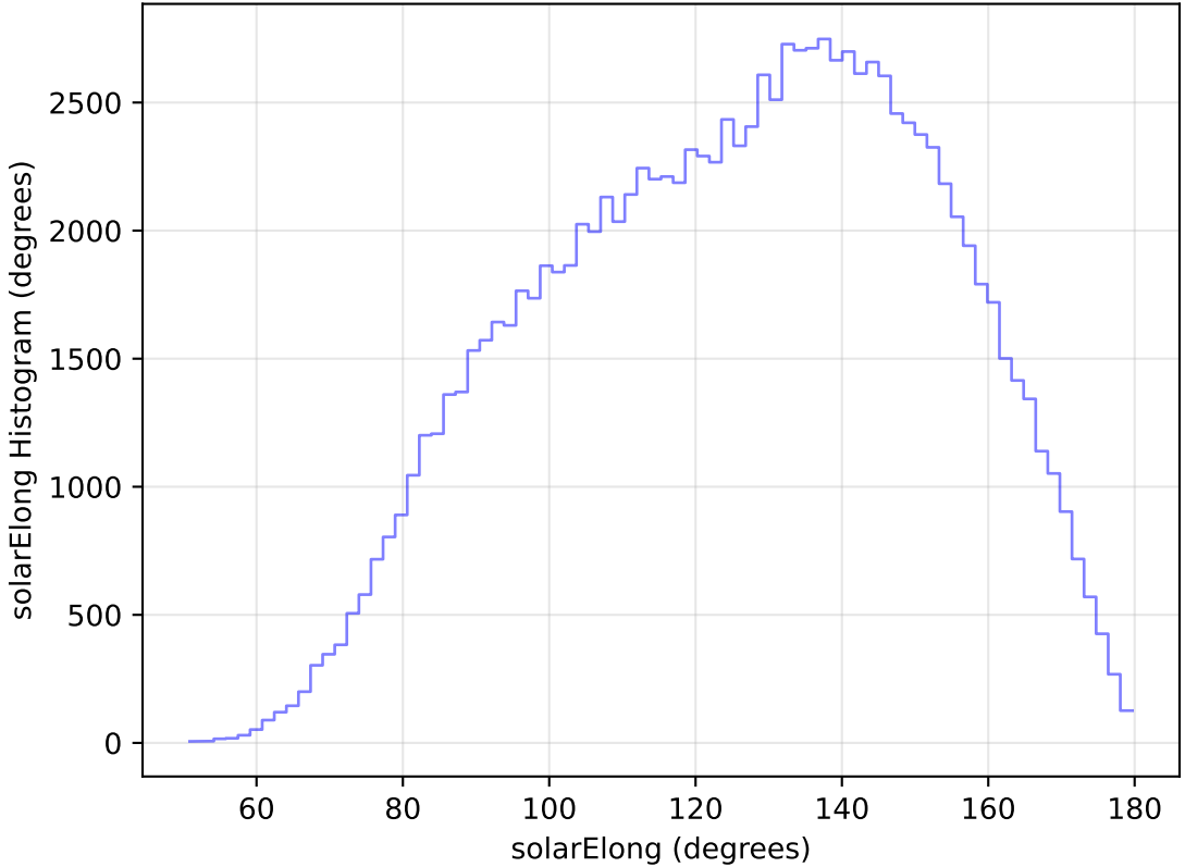
too_elab_heavy_r128_d3_gz_v3.4_10yrs WFD u band: solarElong Histogram
