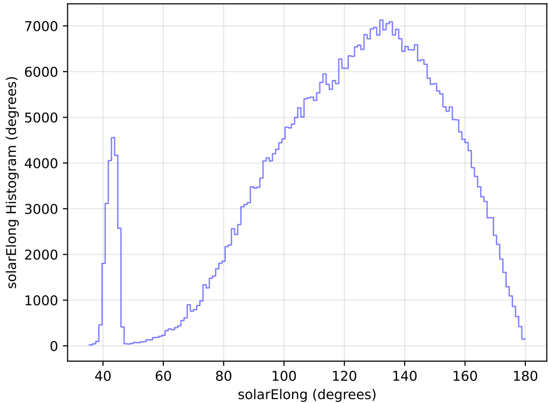
too_elab_heavy_r128_d3_gz_v3.4_10yrs WFD r band: solarElong Histogram
