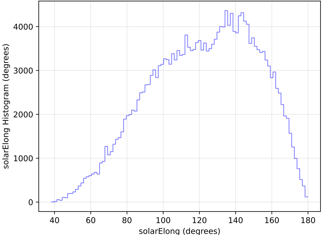
too_elab_heavy_r128_d3_gz_v3.4_10yrs WFD g band: solarElong Histogram
