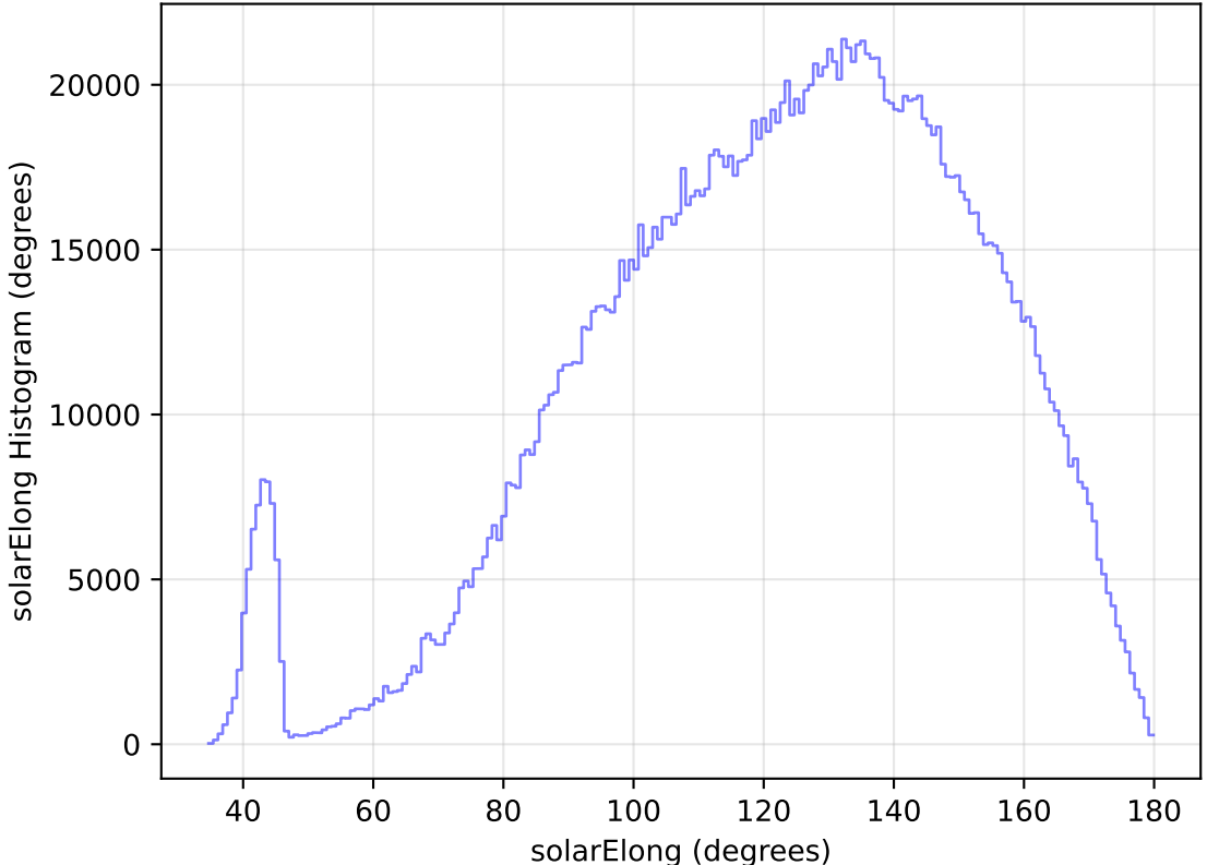
too_elab_heavy_r128_d3_gz_v3.4_10yrs WFD all bands: solarElong Histogram
