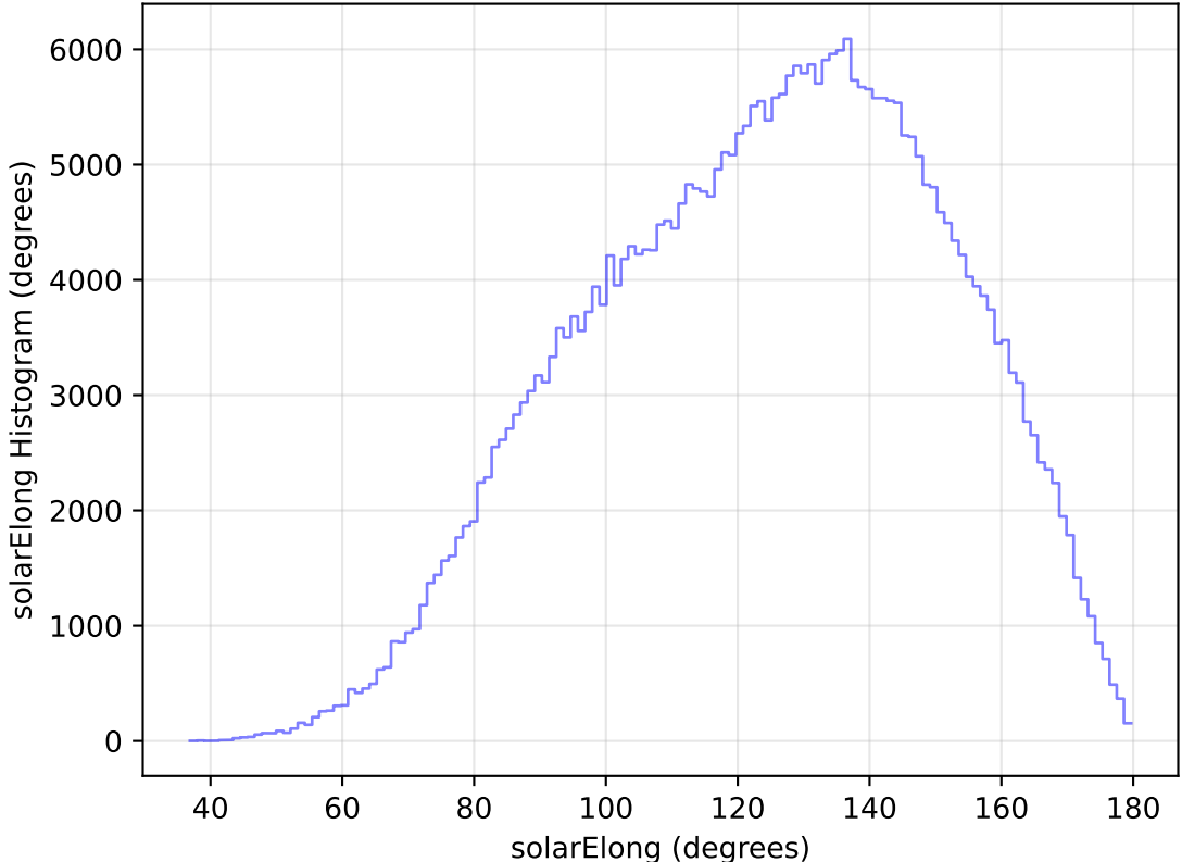
too_elab_heavy_r128_d3_gz_v3.4_10yrs All sky y band: solarElong Histogram
