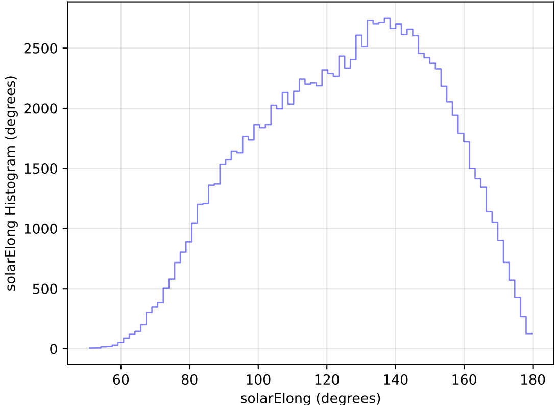
too_elab_heavy_r128_d3_gz_v3.4_10yrs All sky u band: solarElong Histogram
