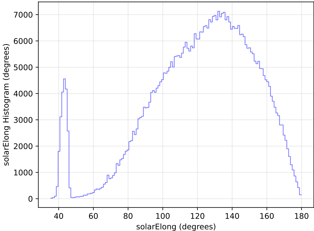
too_elab_heavy_r128_d3_gz_v3.4_10yrs All sky r band: solarElong Histogram
