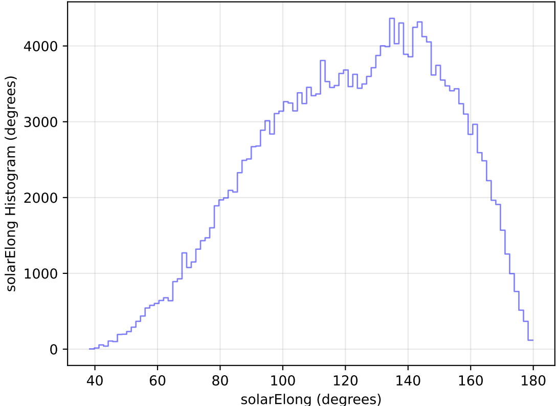
too_elab_heavy_r128_d3_gz_v3.4_10yrs All sky g band: solarElong Histogram
