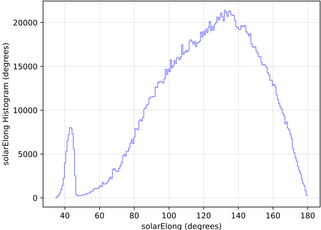
too_elab_heavy_r128_d3_gz_v3.4_10yrs All sky all bands: solarElong Histogram
