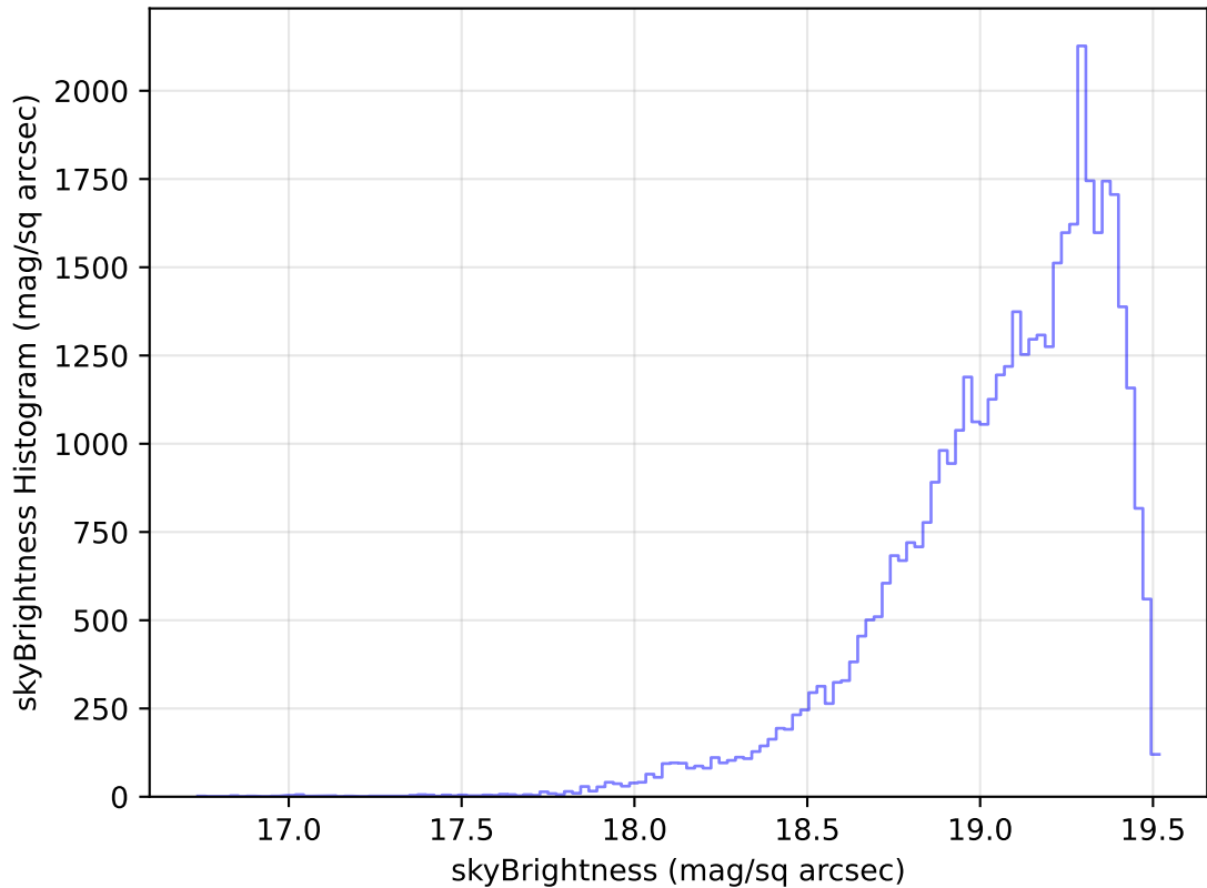
too_elab_heavy_r128_d3_gz_v3.4_10yrs Yr 1 z band: skyBrightness Histogram
