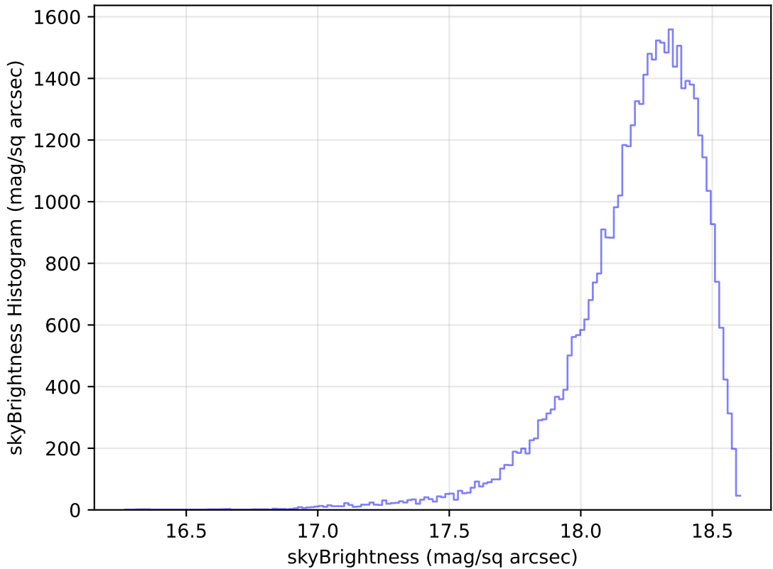
too_elab_heavy_r128_d3_gz_v3.4_10yrs Yr 1 y band: skyBrightness Histogram
