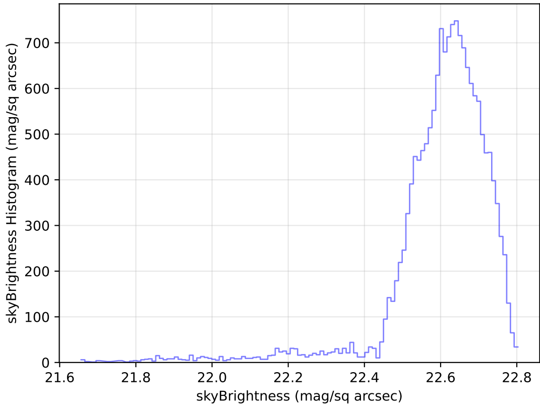
too_elab_heavy_r128_d3_gz_v3.4_10yrs Yr 1 u band: skyBrightness Histogram
