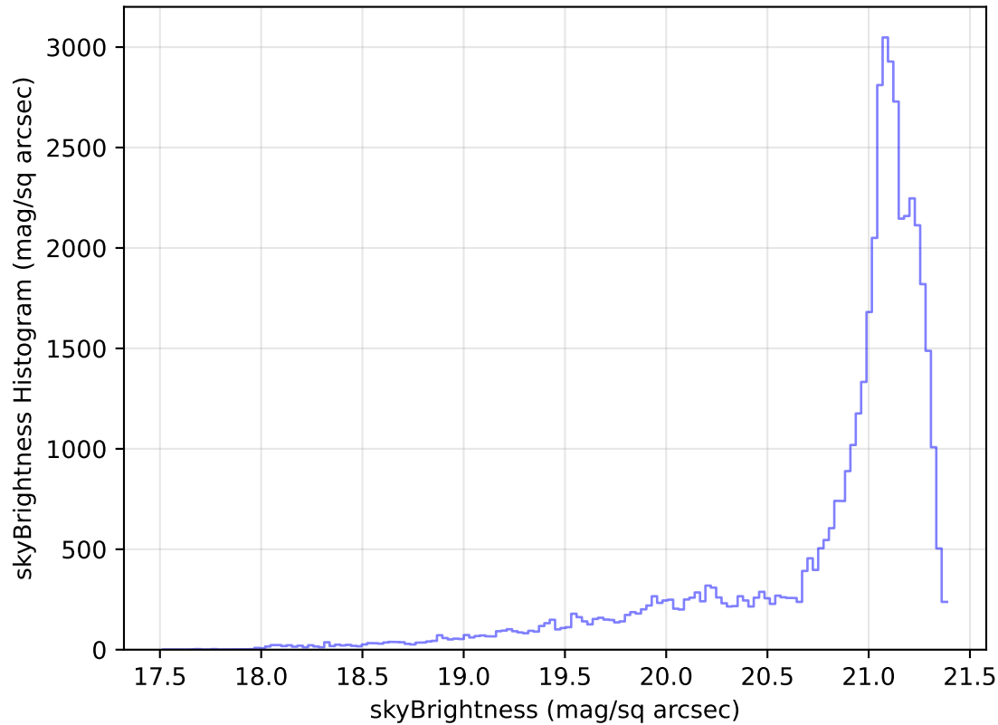
too_elab_heavy_r128_d3_gz_v3.4_10yrs Yr 1 r band: skyBrightness Histogram
