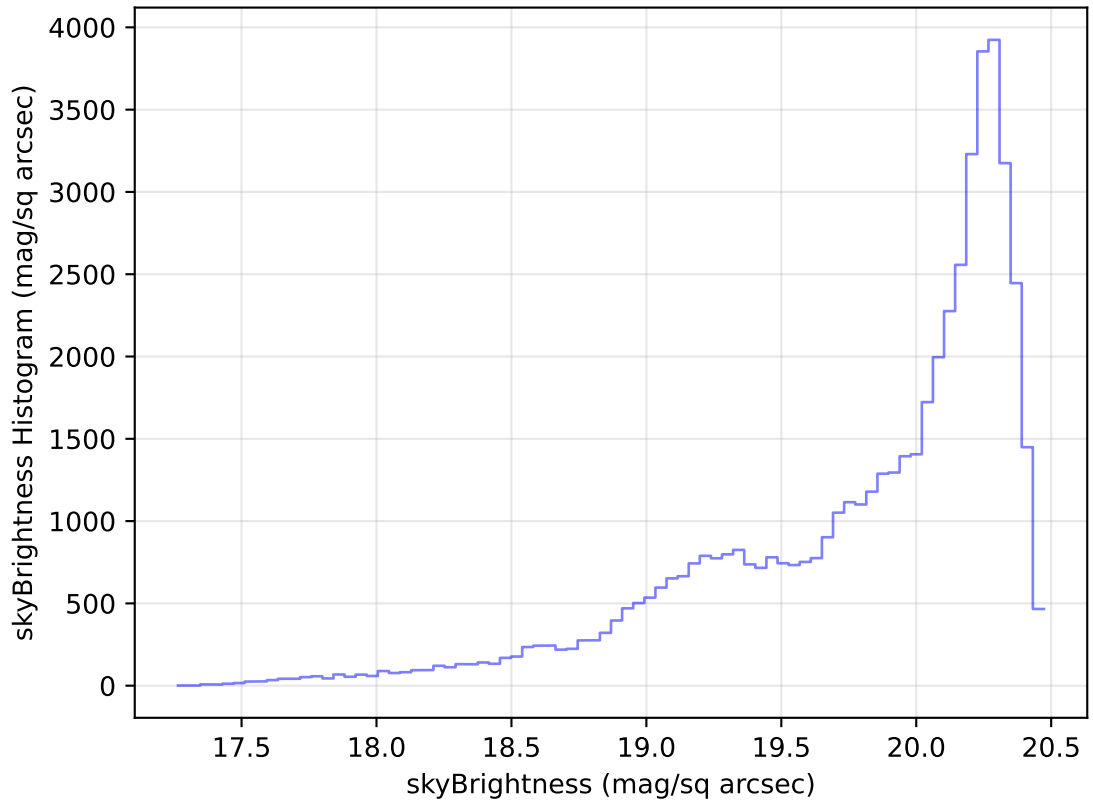
too_elab_heavy_r128_d3_gz_v3.4_10yrs Yr 1 i band: skyBrightness Histogram
