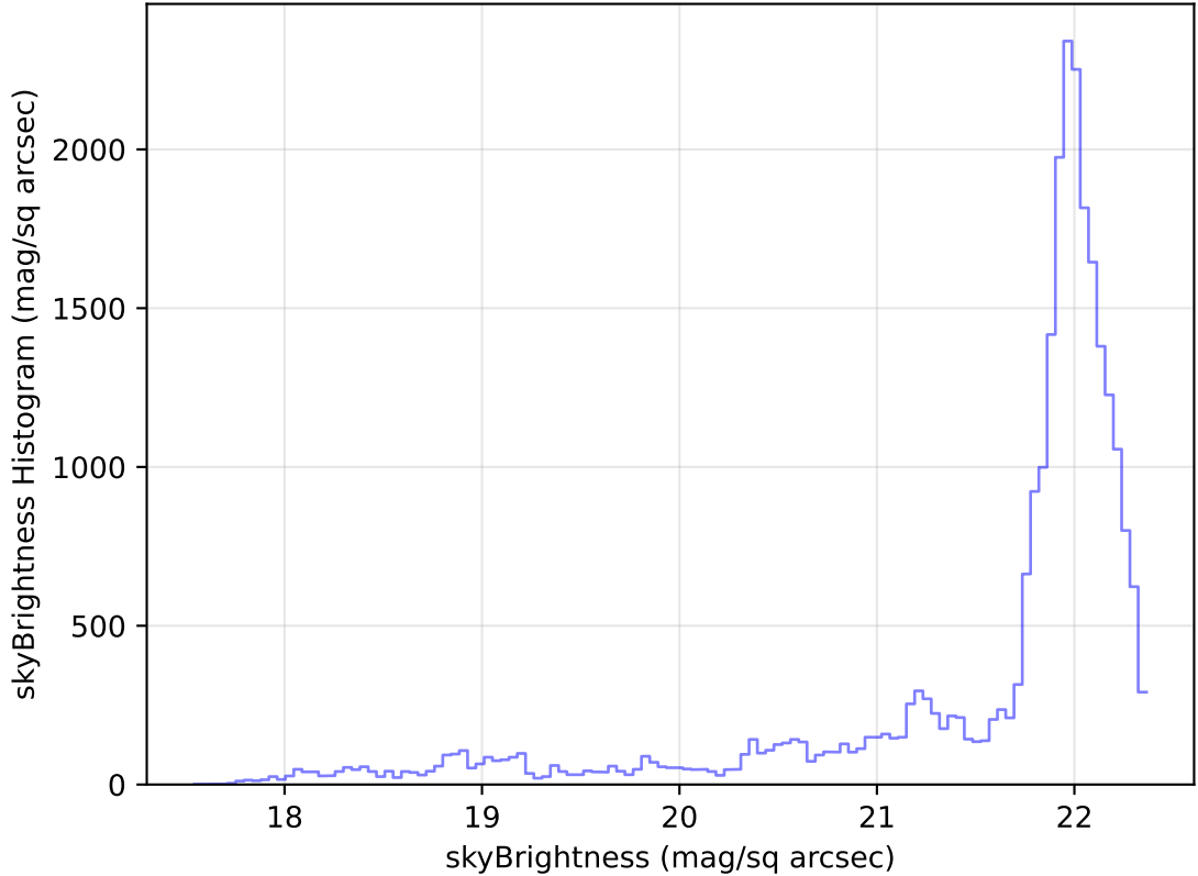
too_elab_heavy_r128_d3_gz_v3.4_10yrs Yr 1 g band: skyBrightness Histogram
