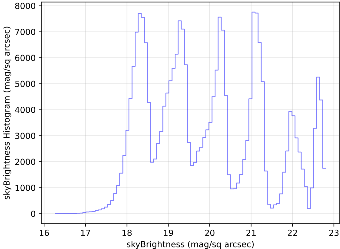
too_elab_heavy_r128_d3_gz_v3.4_10yrs Yr 1 all bands: skyBrightness Histogram
