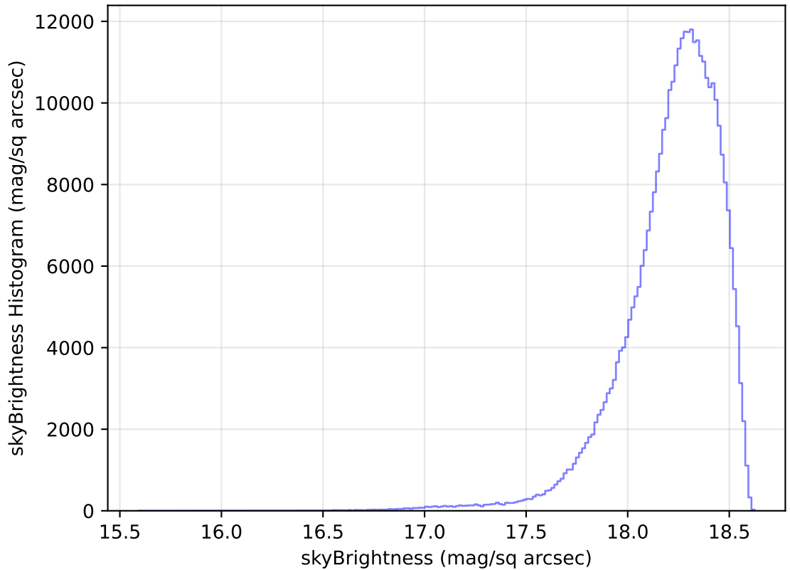
too_elab_heavy_r128_d3_gz_v3.4_10yrs WFD y band: skyBrightness Histogram
