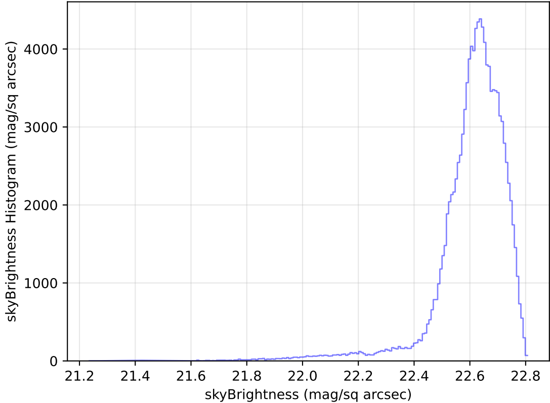
too_elab_heavy_r128_d3_gz_v3.4_10yrs WFD u band: skyBrightness Histogram
