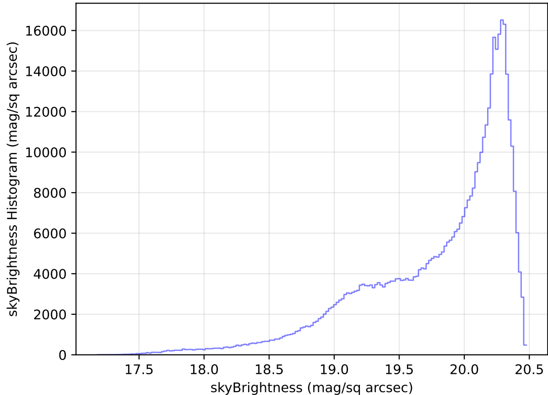
too_elab_heavy_r128_d3_gz_v3.4_10yrs WFD i band: skyBrightness Histogram
