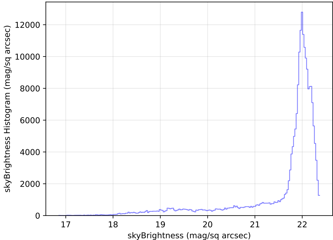
too_elab_heavy_r128_d3_gz_v3.4_10yrs WFD g band: skyBrightness Histogram
