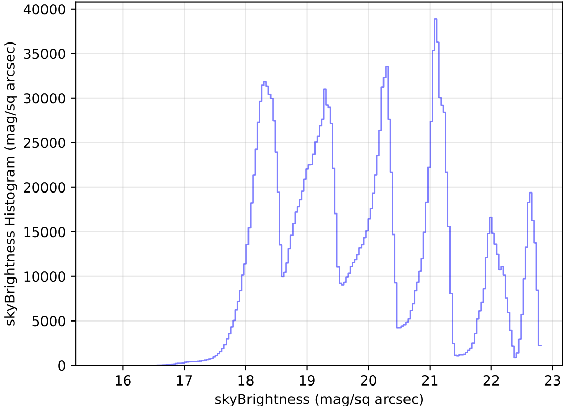
too_elab_heavy_r128_d3_gz_v3.4_10yrs WFD all bands: skyBrightness Histogram
