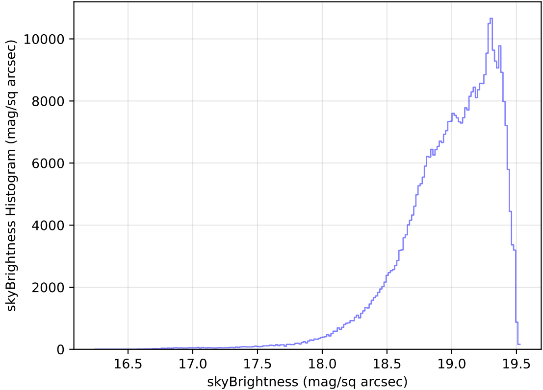
too_elab_heavy_r128_d3_gz_v3.4_10yrs All sky z band: skyBrightness Histogram
