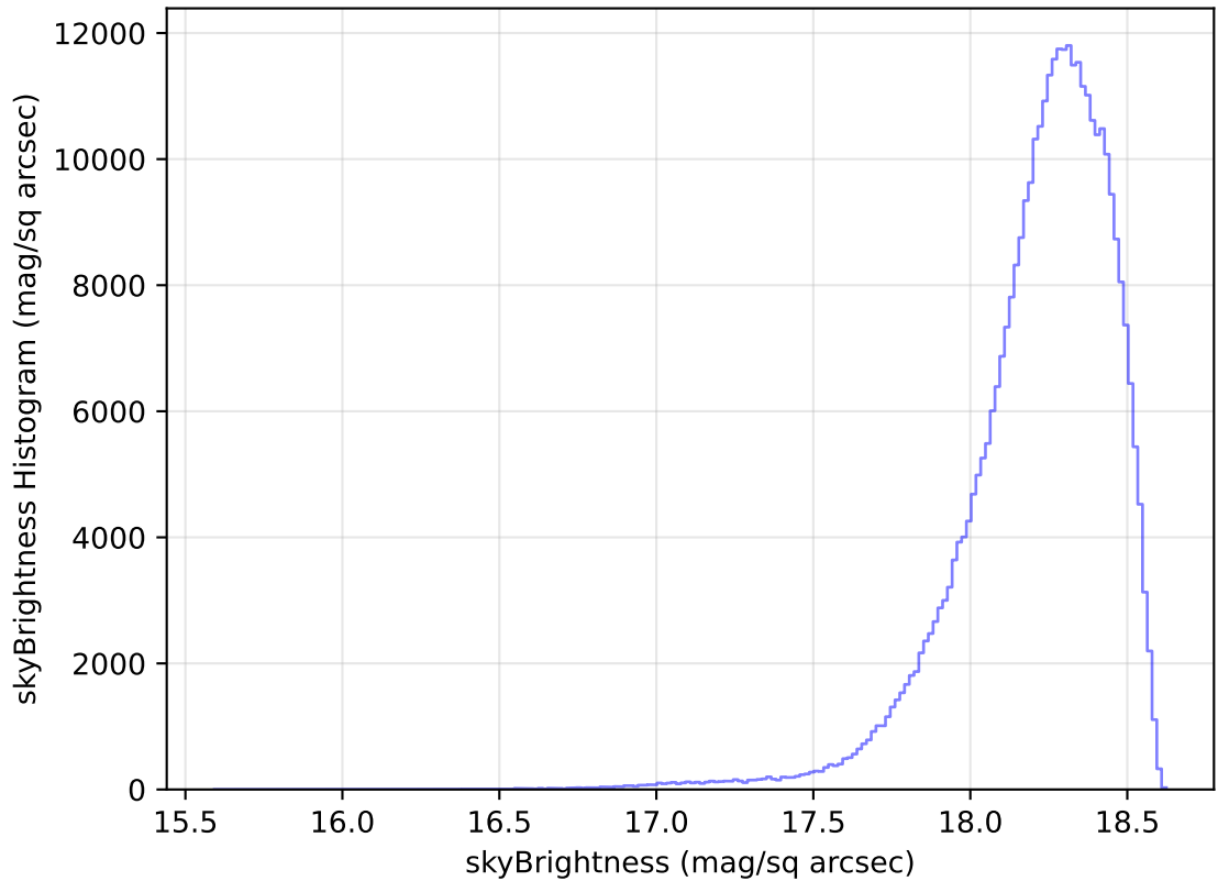
too_elab_heavy_r128_d3_gz_v3.4_10yrs All sky y band: skyBrightness Histogram
