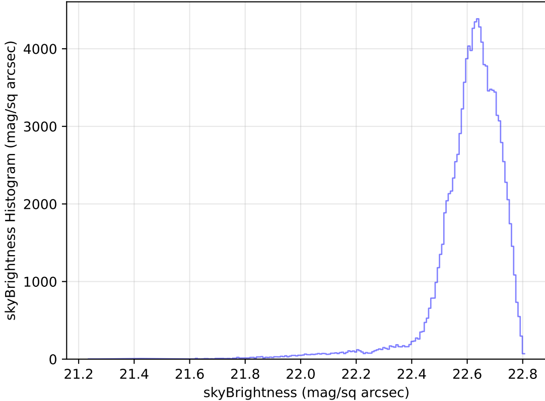
too_elab_heavy_r128_d3_gz_v3.4_10yrs All sky u band: skyBrightness Histogram
