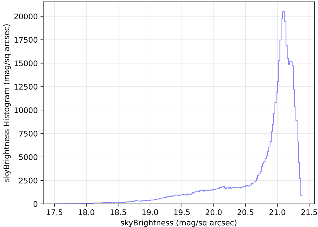
too_elab_heavy_r128_d3_gz_v3.4_10yrs All sky r band: skyBrightness Histogram
