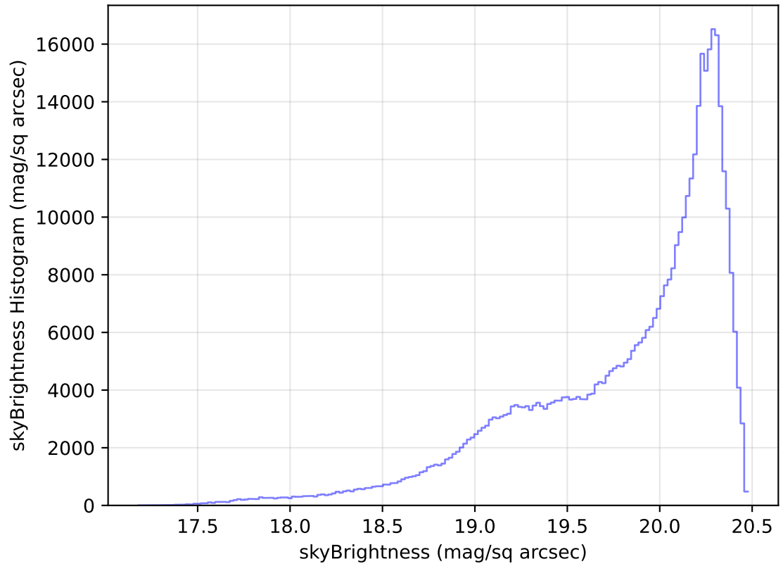
too_elab_heavy_r128_d3_gz_v3.4_10yrs All sky i band: skyBrightness Histogram
