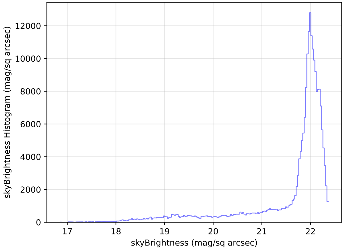
too_elab_heavy_r128_d3_gz_v3.4_10yrs All sky g band: skyBrightness Histogram
