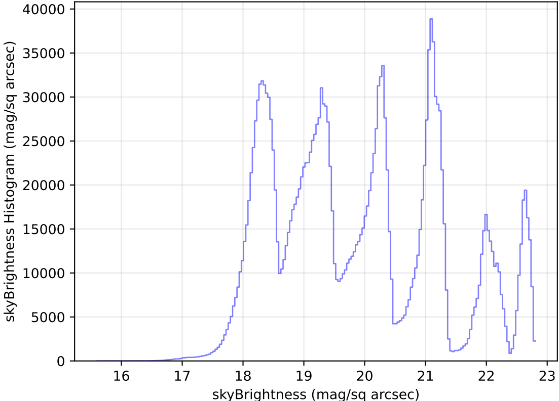
too_elab_heavy_r128_d3_gz_v3.4_10yrs All sky all bands: skyBrightness Histogram
