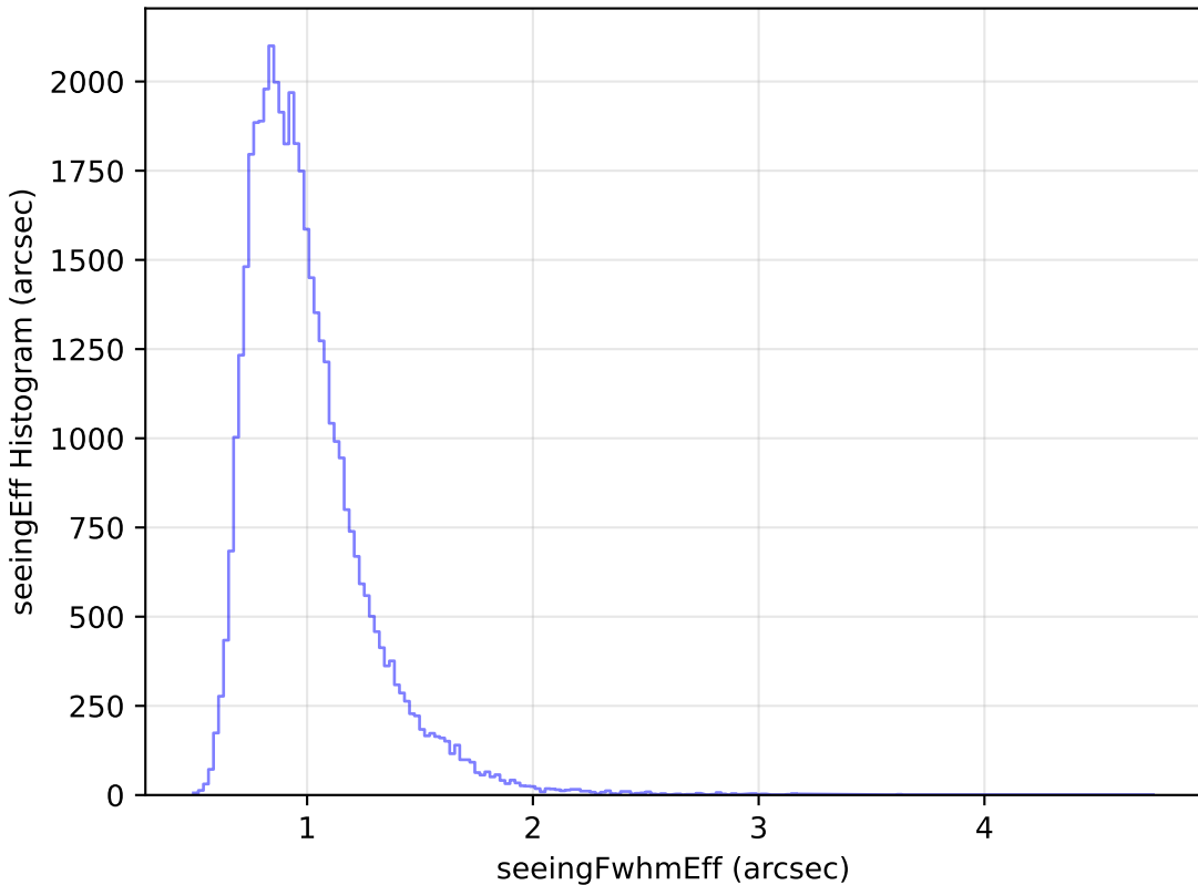
too_elab_heavy_r128_d3_gz_v3.4_10yrs Yr 1 z band: seeingEff Histogram
