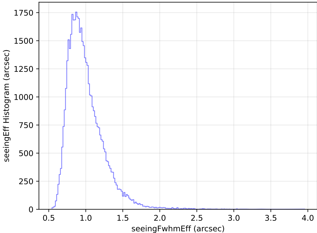
too_elab_heavy_r128_d3_gz_v3.4_10yrs Yr 1 y band: seeingEff Histogram
