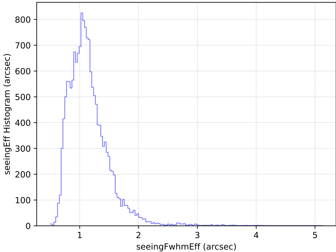
too_elab_heavy_r128_d3_gz_v3.4_10yrs Yr 1 u band: seeingEff Histogram
