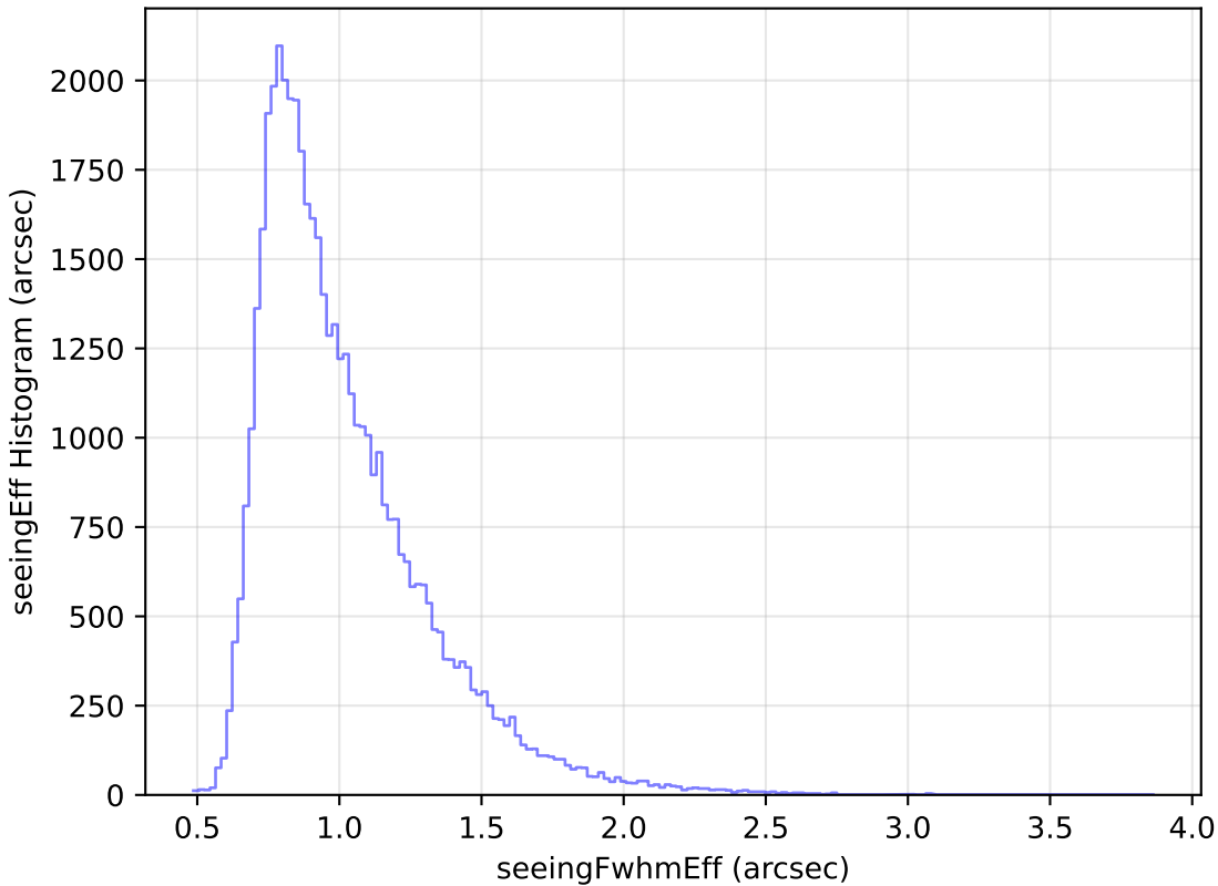
too_elab_heavy_r128_d3_gz_v3.4_10yrs Yr 1 r band: seeingEff Histogram
