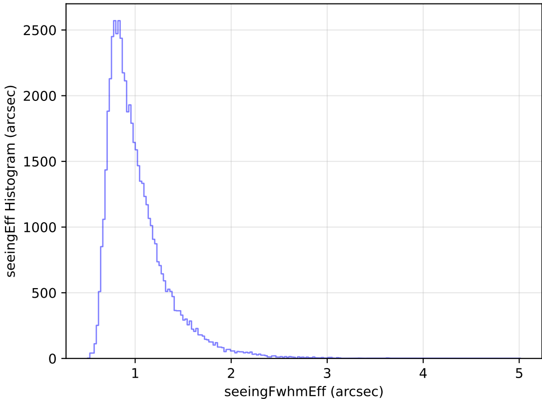
too_elab_heavy_r128_d3_gz_v3.4_10yrs Yr 1 i band: seeingEff Histogram
