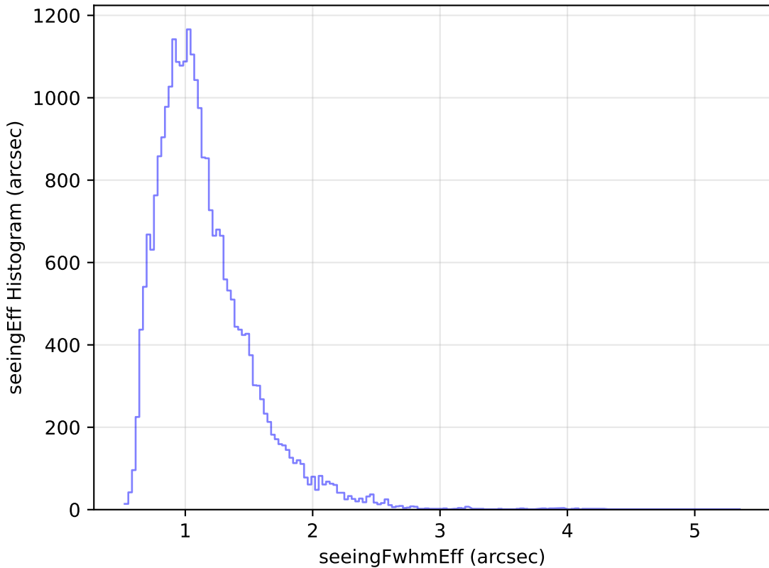
too_elab_heavy_r128_d3_gz_v3.4_10yrs Yr 1 g band: seeingEff Histogram
