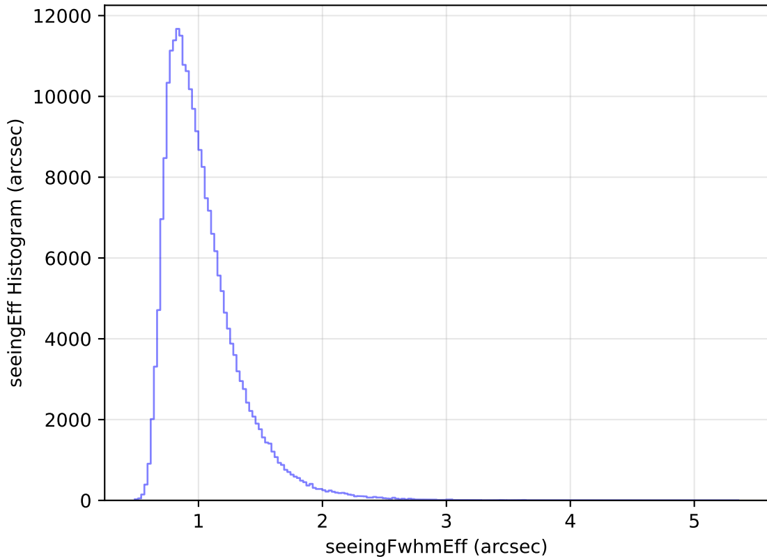
too_elab_heavy_r128_d3_gz_v3.4_10yrs Yr 1 all bands: seeingEff Histogram
