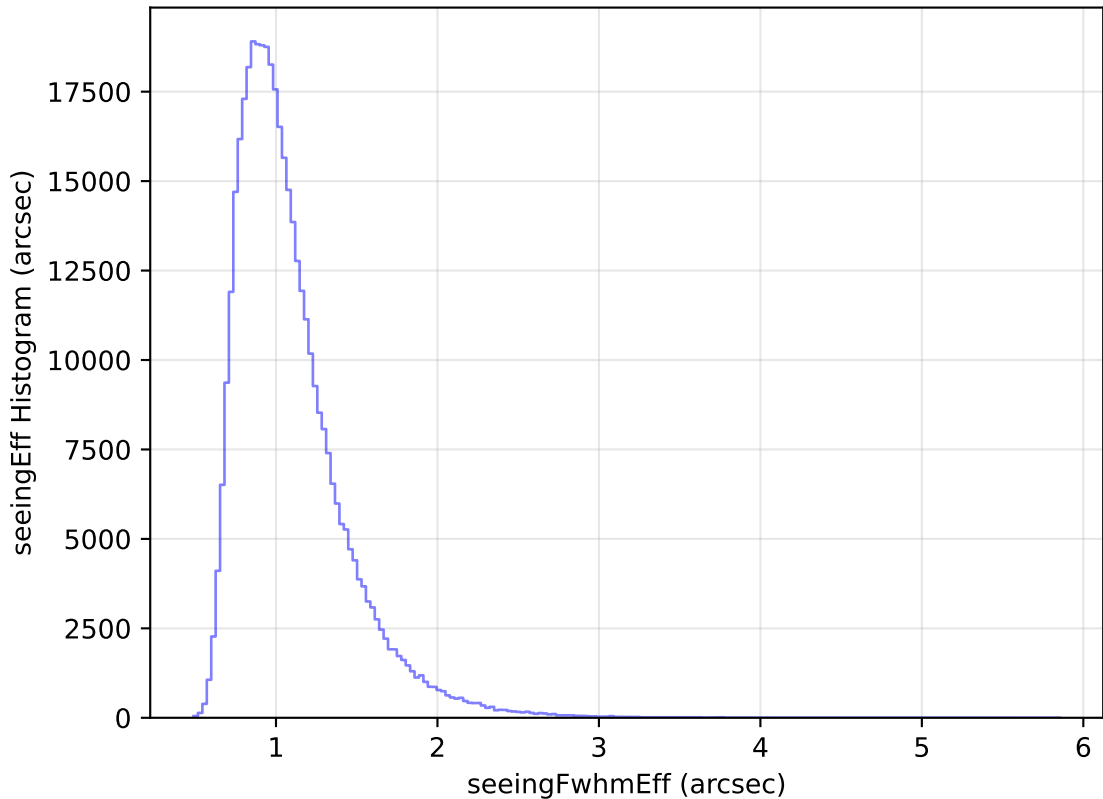
too_elab_heavy_r128_d3_gz_v3.4_10yrs WFD z band: seeingEff Histogram
