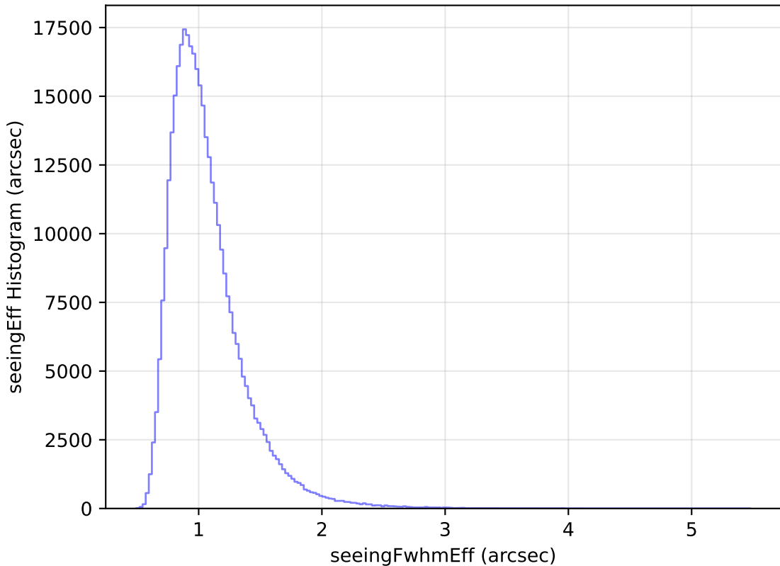
too_elab_heavy_r128_d3_gz_v3.4_10yrs WFD y band: seeingEff Histogram
