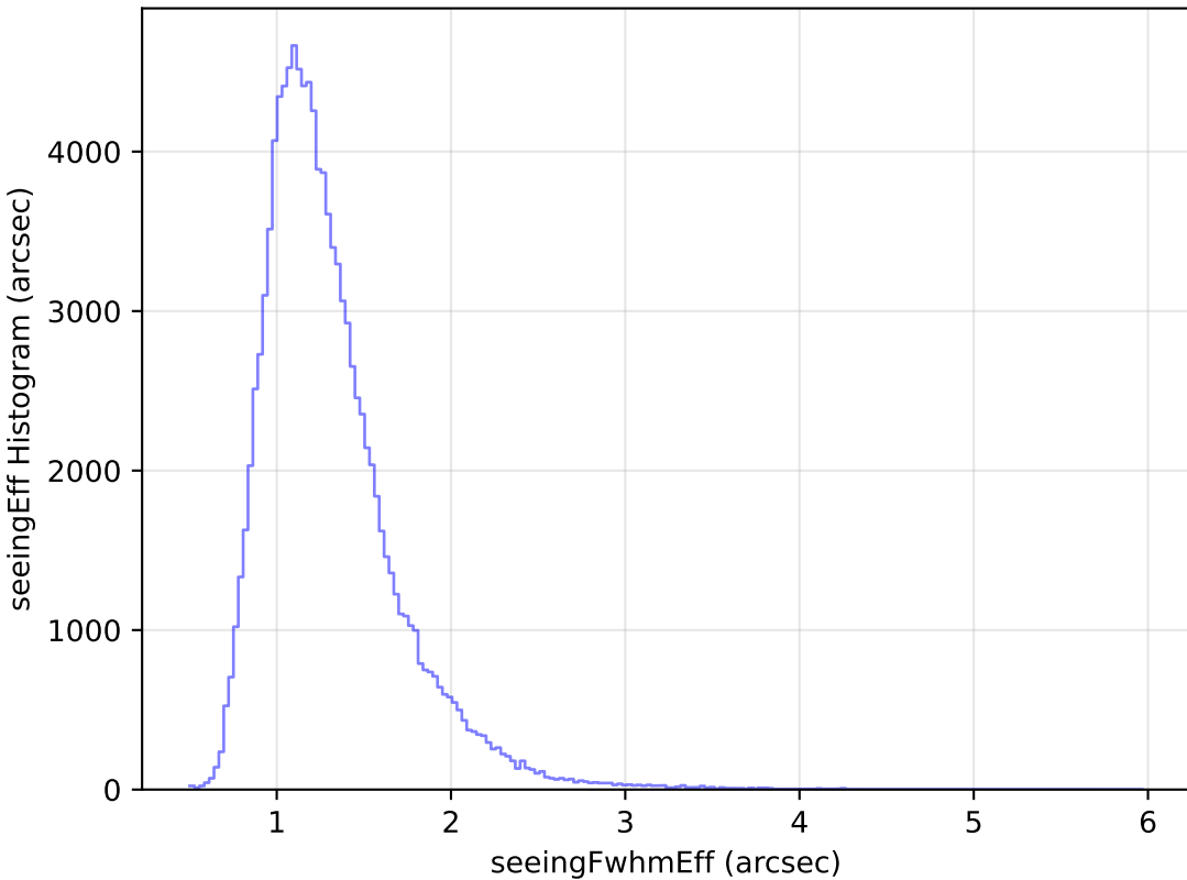
too_elab_heavy_r128_d3_gz_v3.4_10yrs WFD u band: seeingEff Histogram
