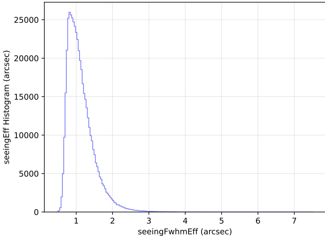
too_elab_heavy_r128_d3_gz_v3.4_10yrs WFD r band: seeingEff Histogram
