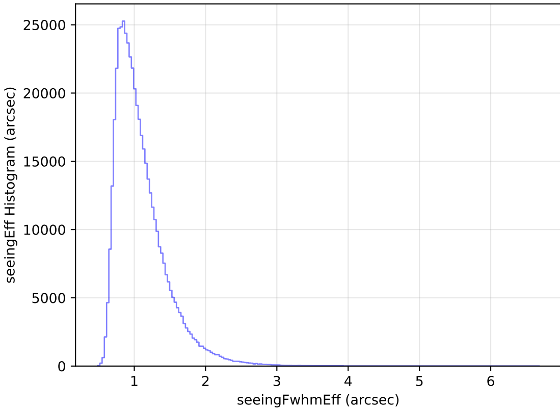
too_elab_heavy_r128_d3_gz_v3.4_10yrs WFD i band: seeingEff Histogram
